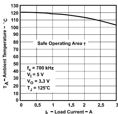
AMBIENT TEMPERATURE vs LOAD CURRENT
